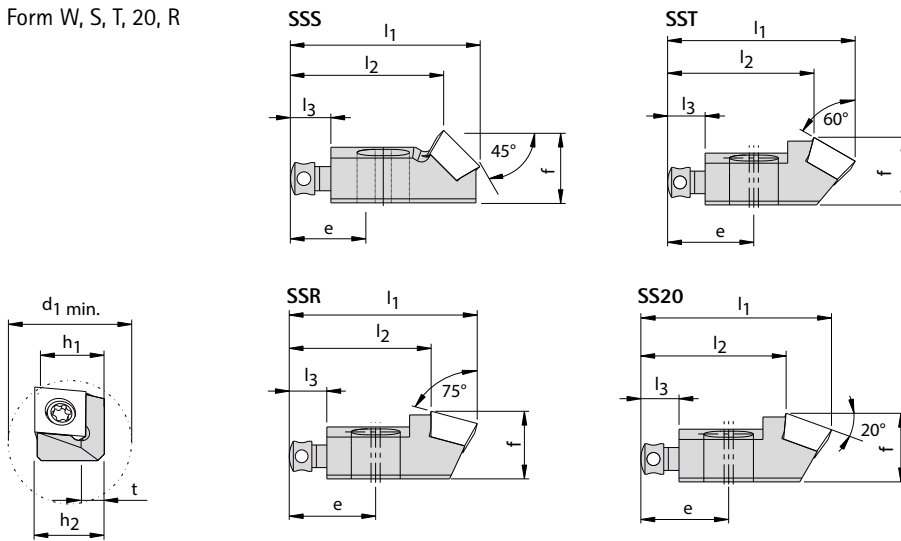
Drawings of right design, example SSSDR.
