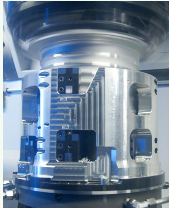
The difference in the tool speed and the workpiece speed produces the cutting speed at the inner blades. The bell-shaped outer tool stands still.
