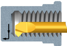
Chamfering & Boring
